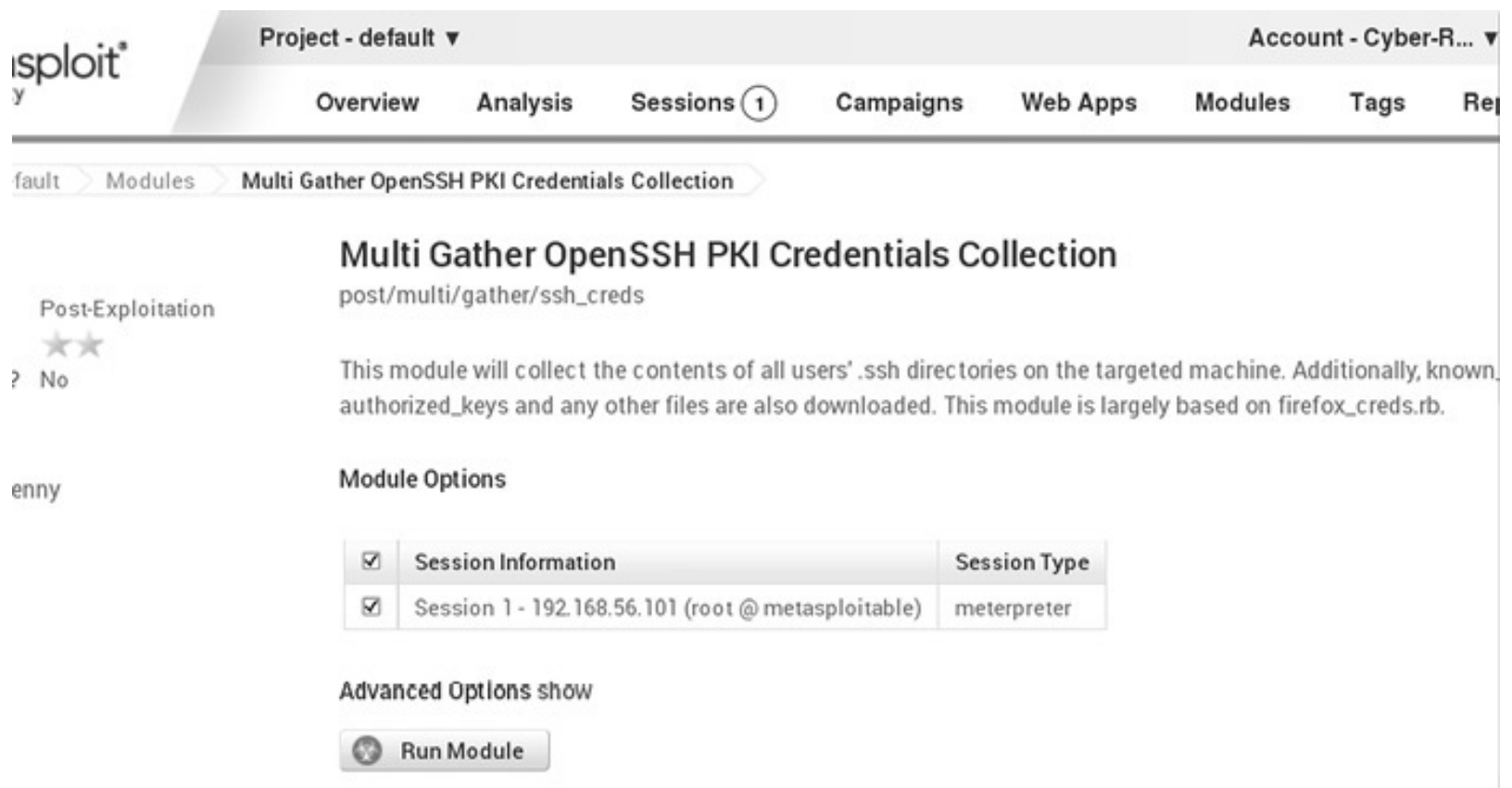
Figura 9.16 – Multi Gather OpenSSH PKI.
